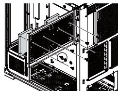
SSD Screw
